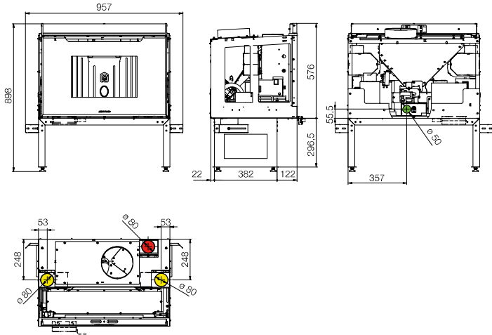
SYNTHESIS MODULAR 80
